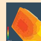
Thermal simulation results of LED-based street-lighting luminaire
